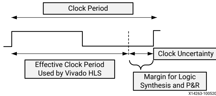
Figure 22: Clock Period and Margin
