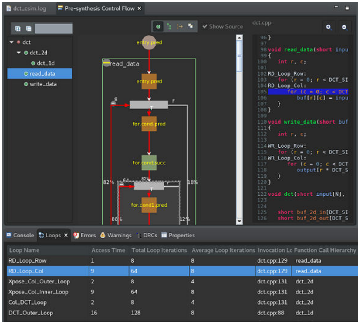
Figure 28: Pre-Synthesis Control Flow Viewer
