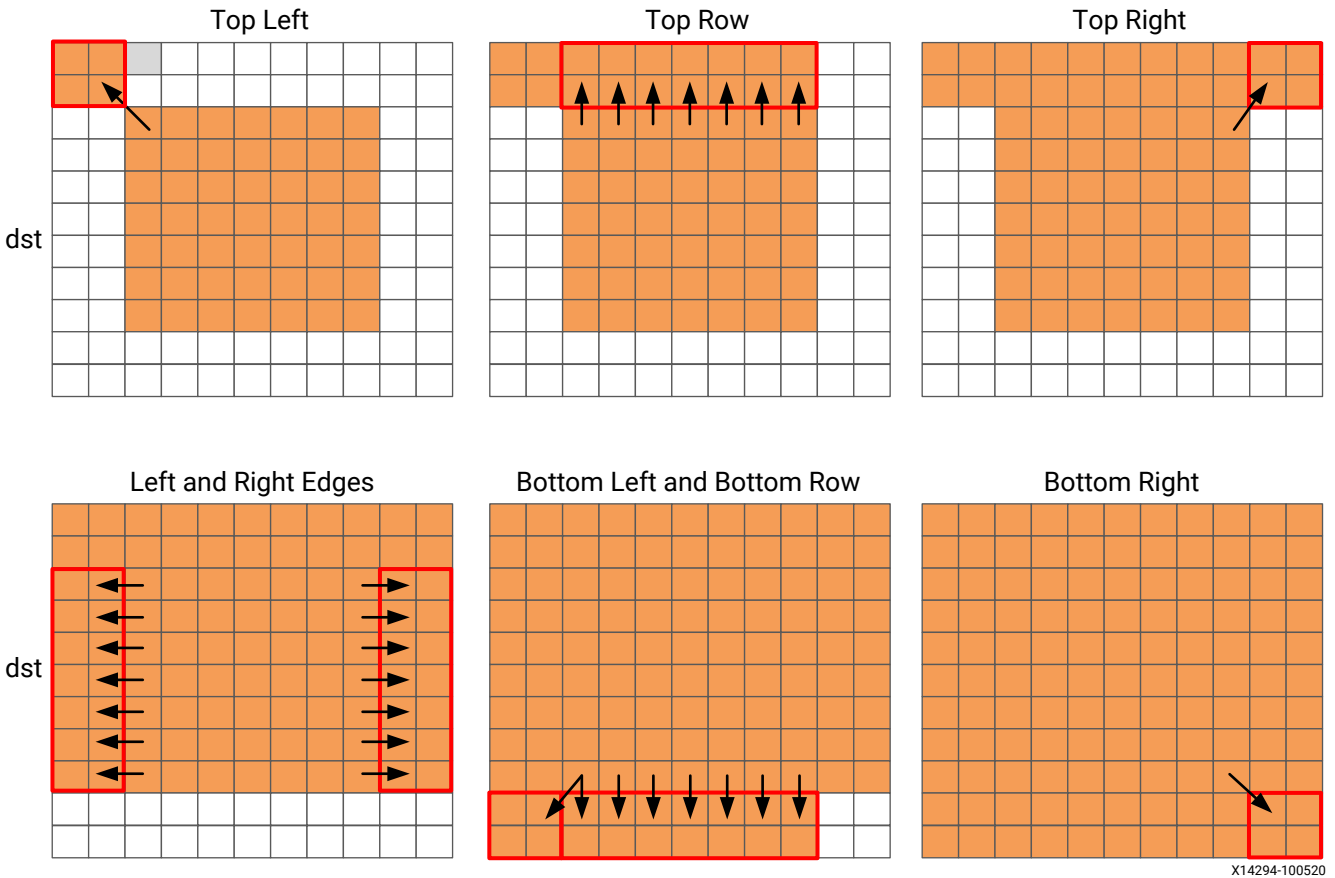
Figure 58: Convolution Border Samples
