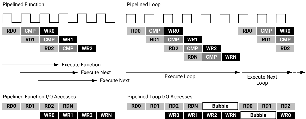
Figure 86: Function and Loop Pipelining Behavior
