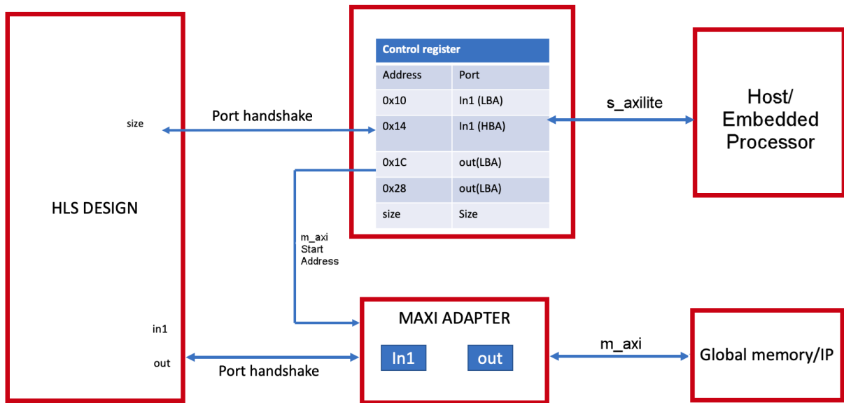
Figure 68: AXI Adapters in Slave Mode
