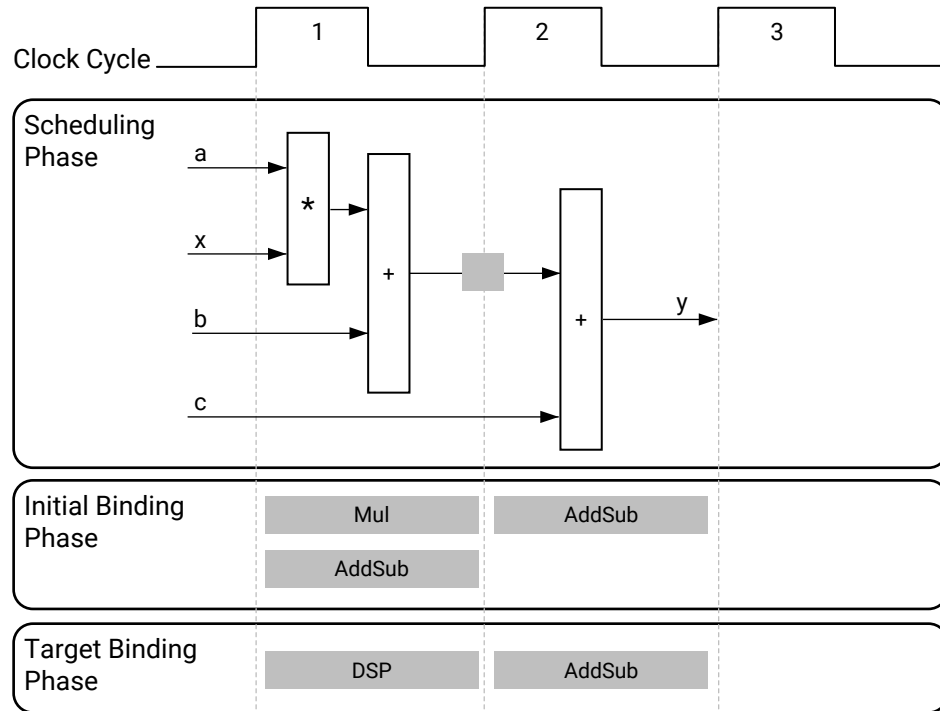
Figure 11: Scheduling and Binding Example
