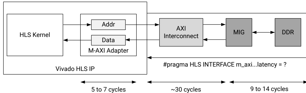
Figure 105: Burst Transaction Diagram
