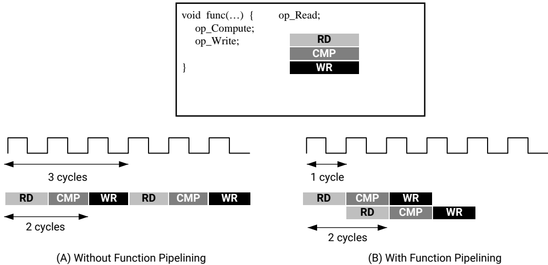
Figure 84: Function Pipelining Behavior
