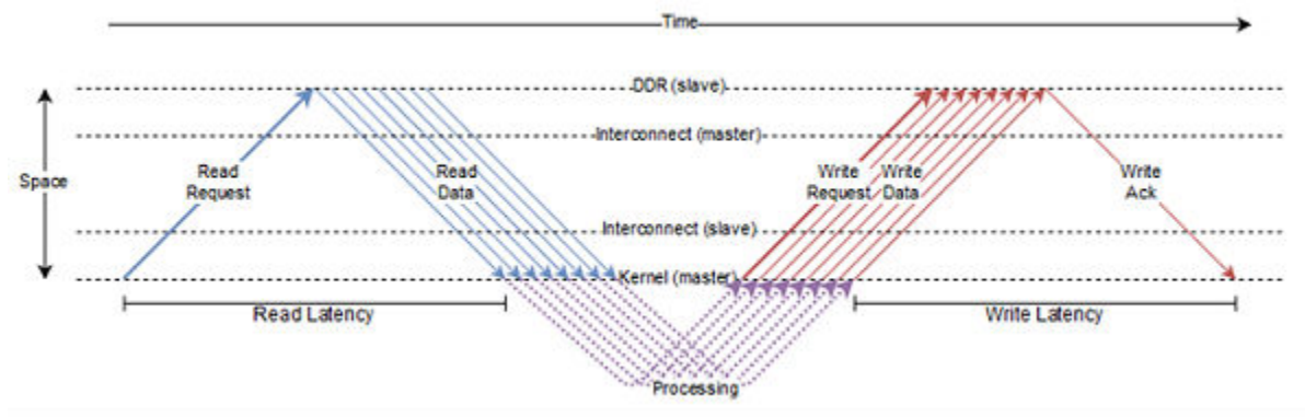
Figure 102: AXI Protocol
