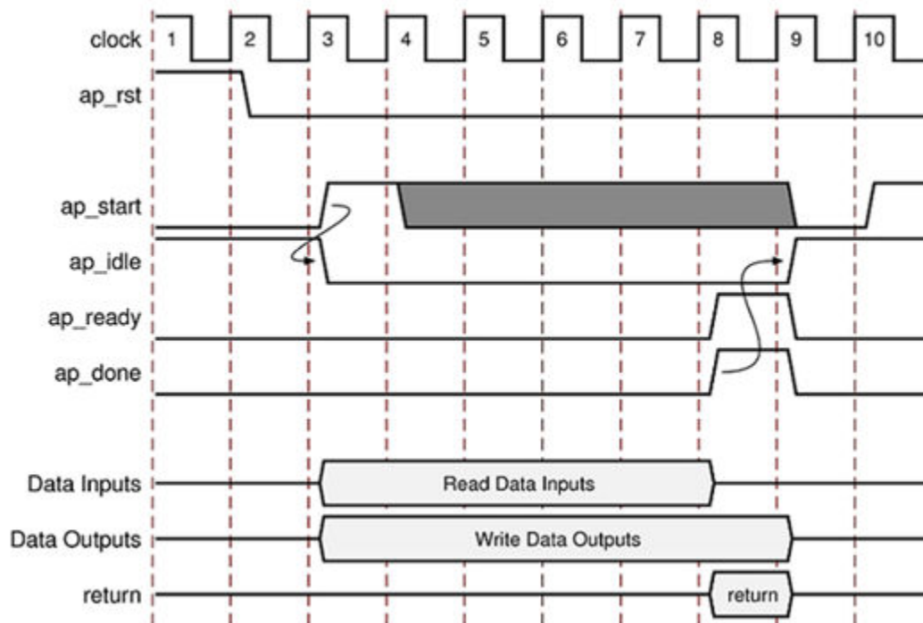
Figure 81: Behavior of ap_ctrl_hs Interface
