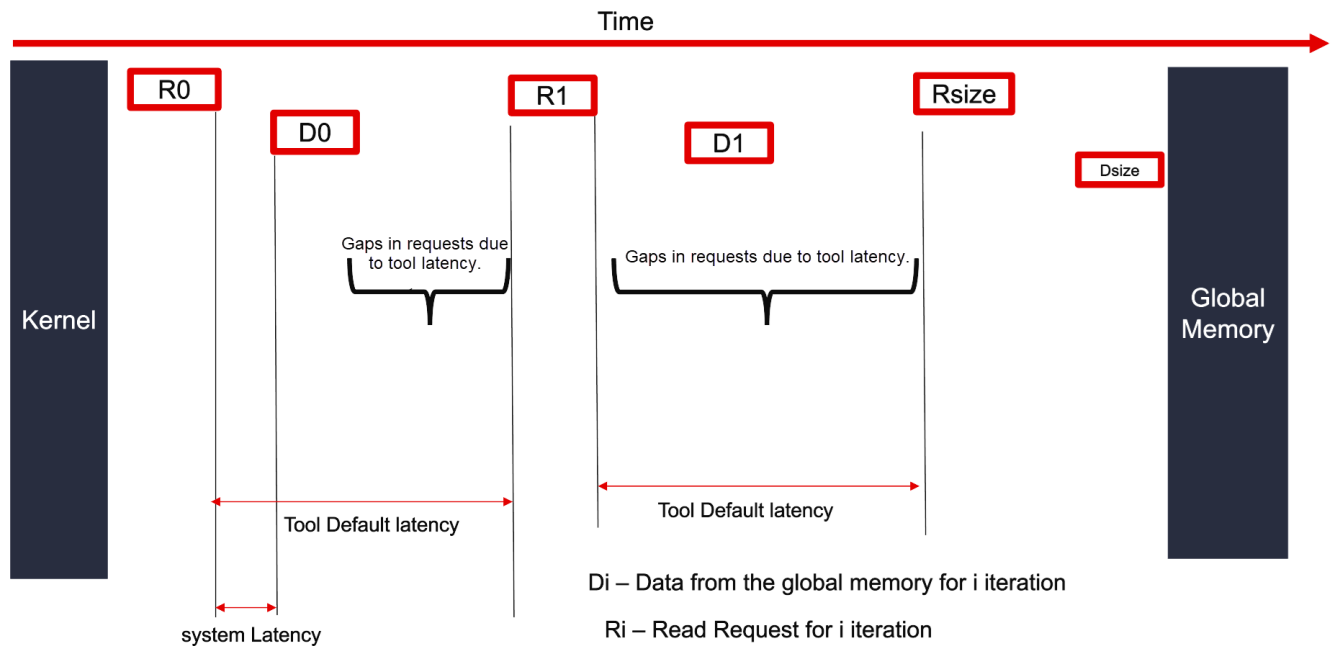
Figure 106: Default Tool Latency
