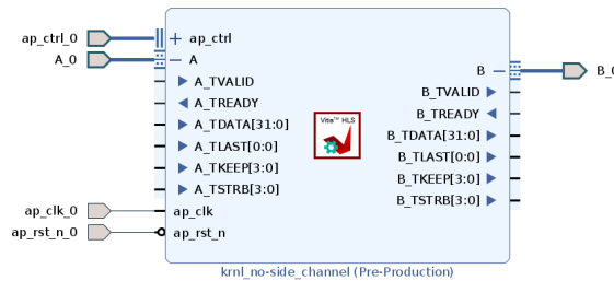
Figure 75: AXI4-Stream Interfaces without Side-Channels
