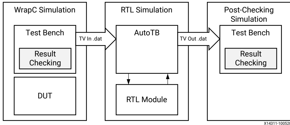
Figure 47: C/RTL Verification Flow
