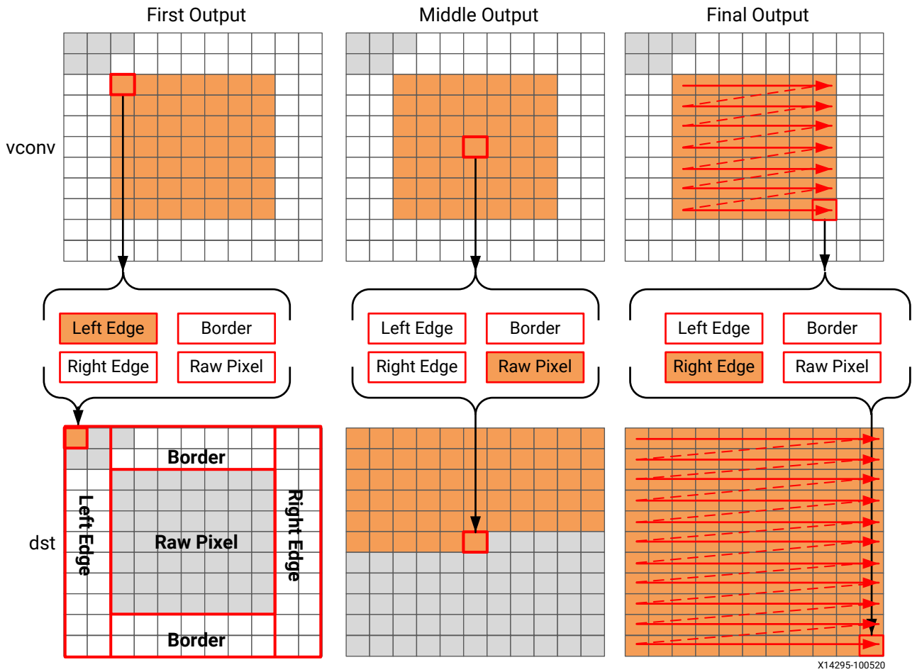
Figure 62: Streaming Border Samples
