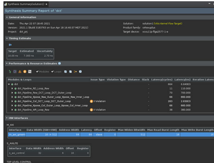
Figure 31: Synthesis Summary Report
