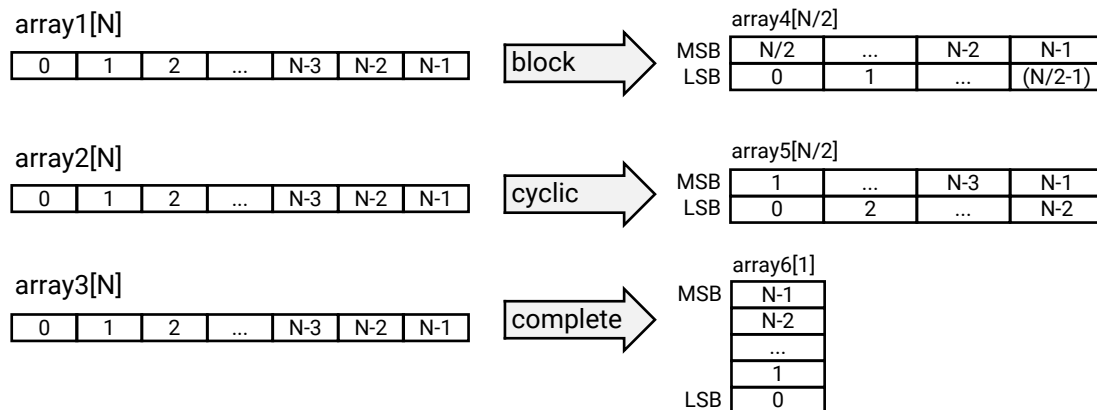
Figure 126: ARRAY_RESHAPE Pragma
