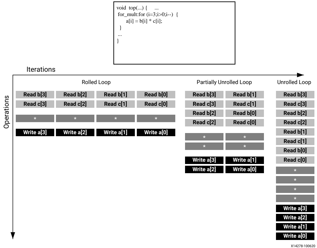
Figure 89: Loop Unrolling Details
