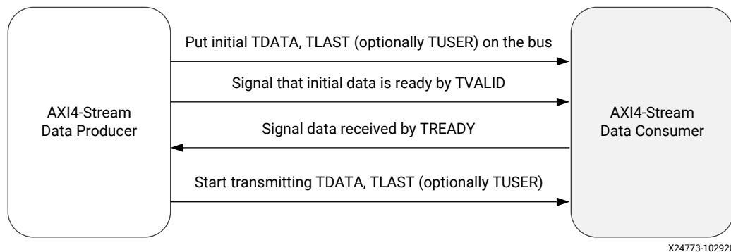
Figure 74: AXI4-Stream Handshake
