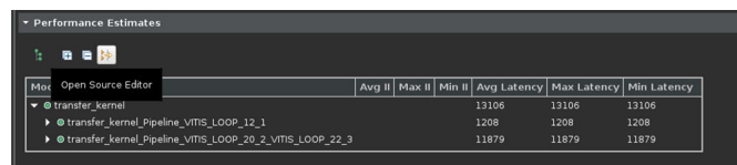
Figure 113: Performance Estimates
