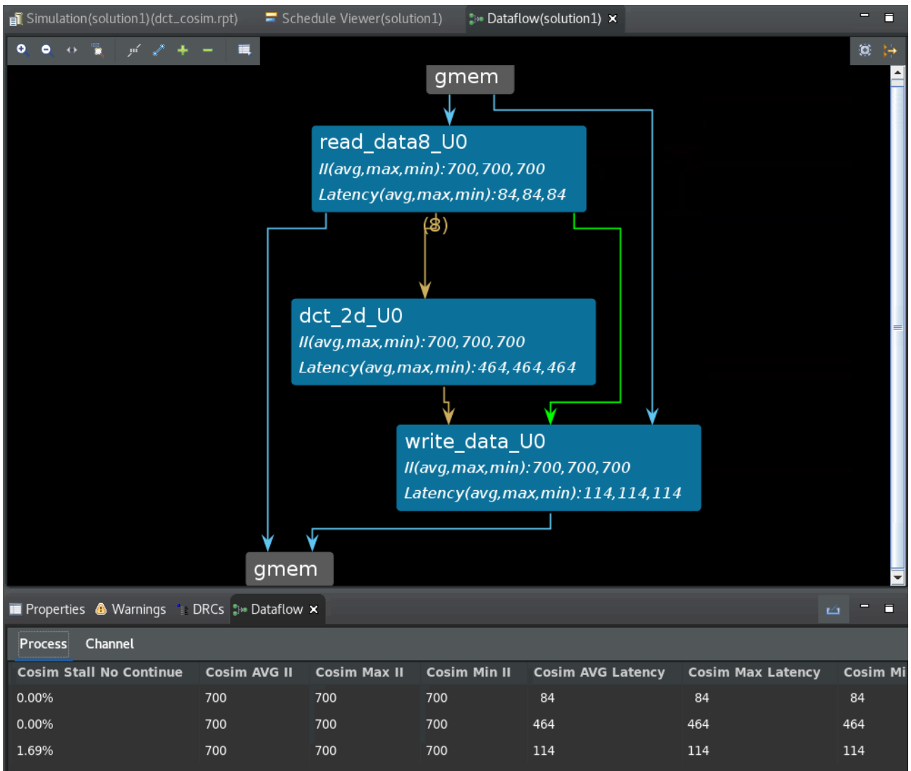
Figure 41: Dataflow Viewer
