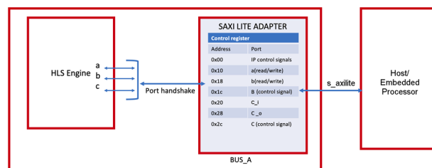
Figure 72: S_AXILITE Adapter
