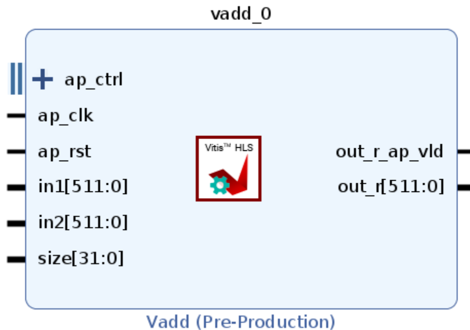
Figure 65: RTL Ports After Default Interface Synthesis
