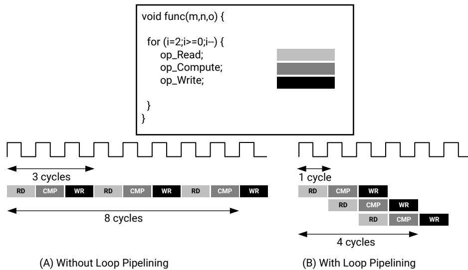
Figure 128: Loop Pipeline
