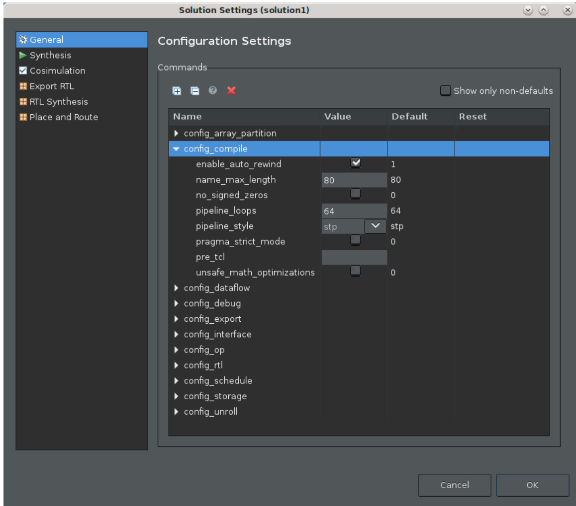
Figure 20: Solution Settings Dialog Box
