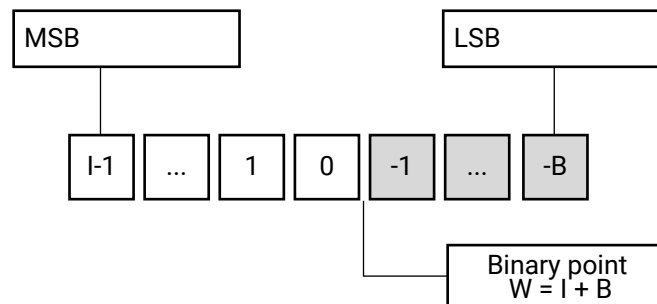
Figure 129: Fixed-Point Data Type
