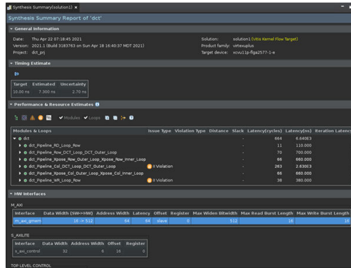
Figure 29: Synthesis Summary Report
