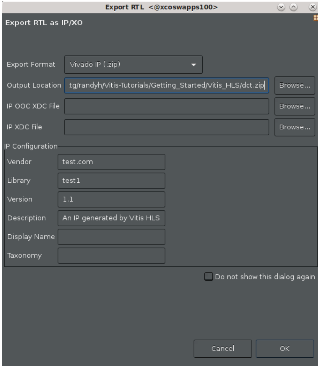
Figure 50: Export RTL Dialog Box
