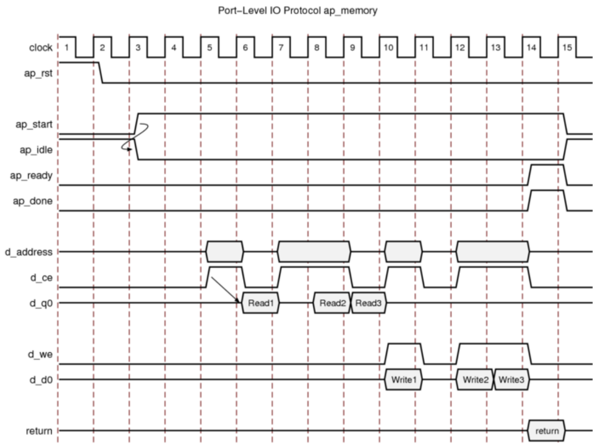
Figure 79: Behavior of ap_memory Interface
