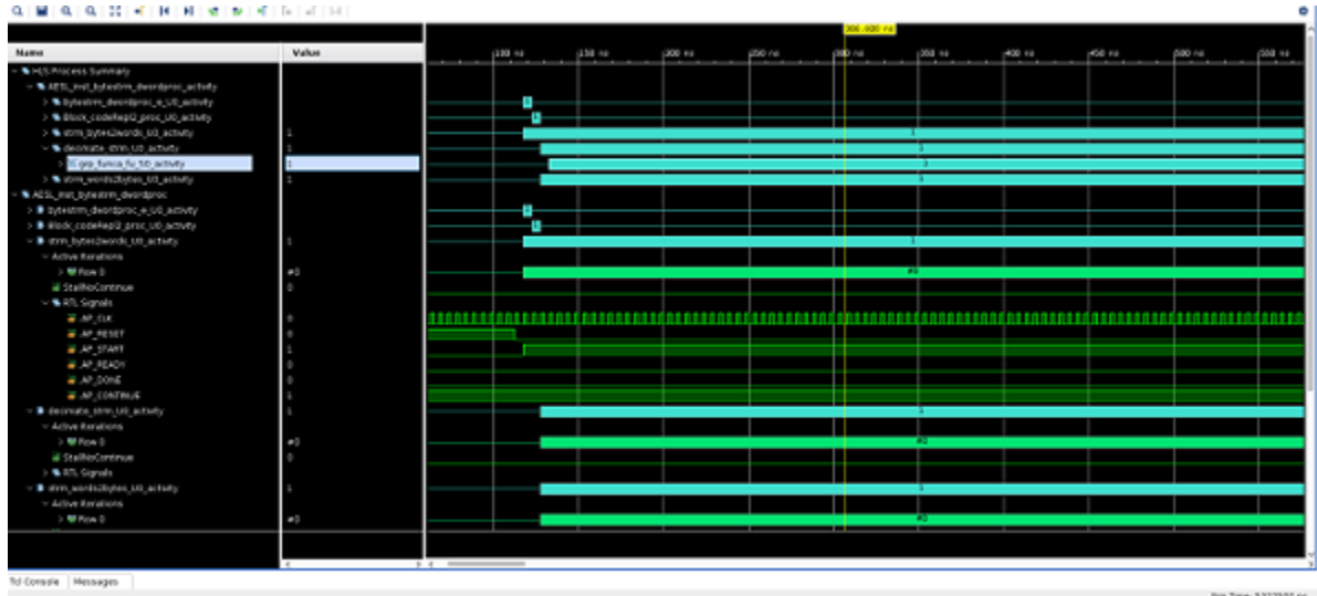
Figure 48: Waveform Viewer
