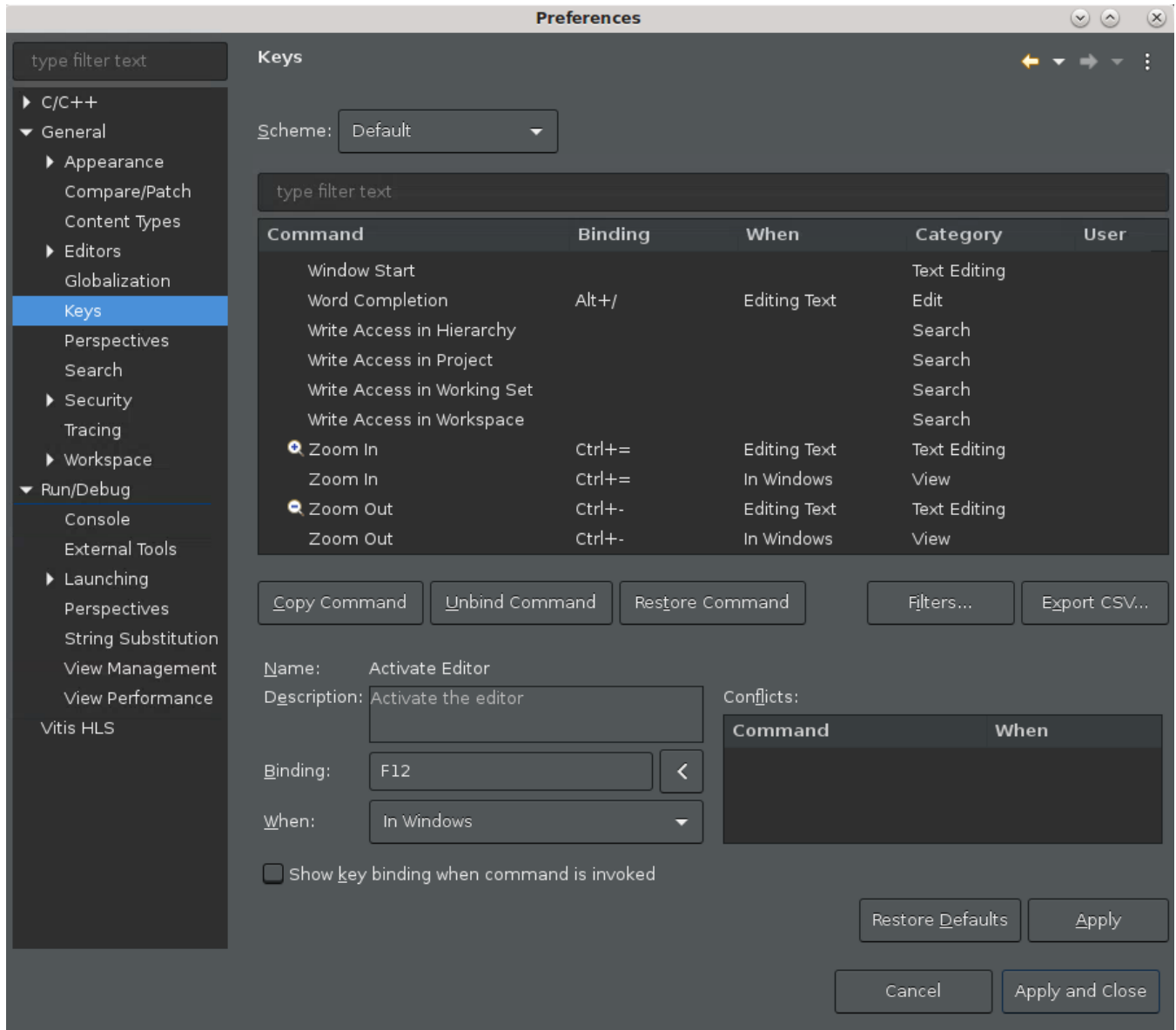
Figure 16: Keyboard Shortcuts
