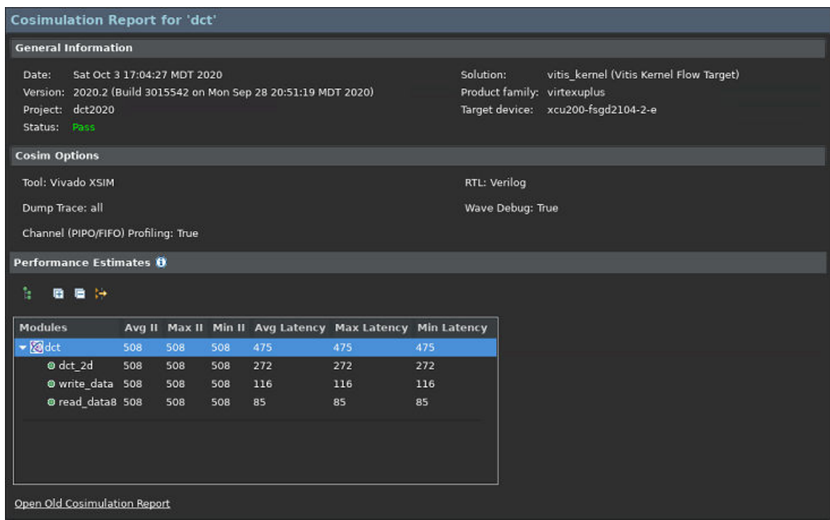
Figure 46: Cosimulation Report
