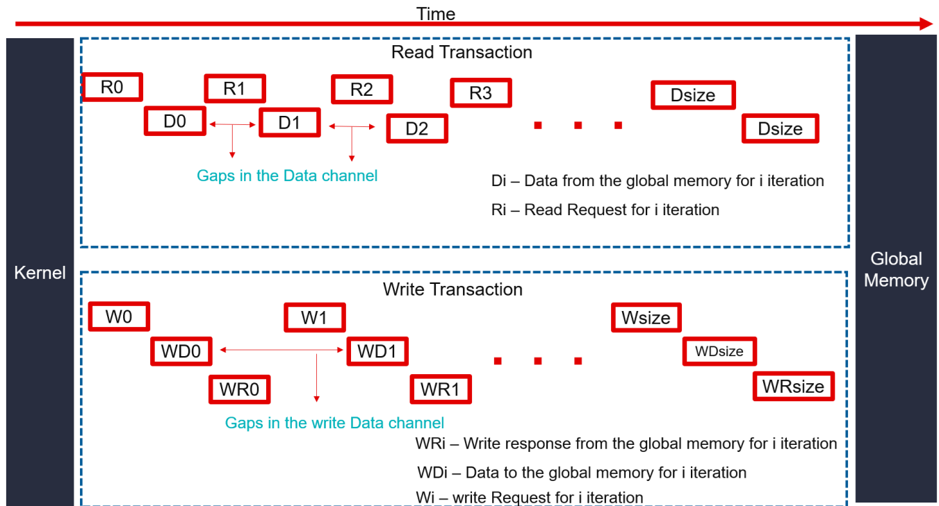
Figure 104: Sequential Burst
