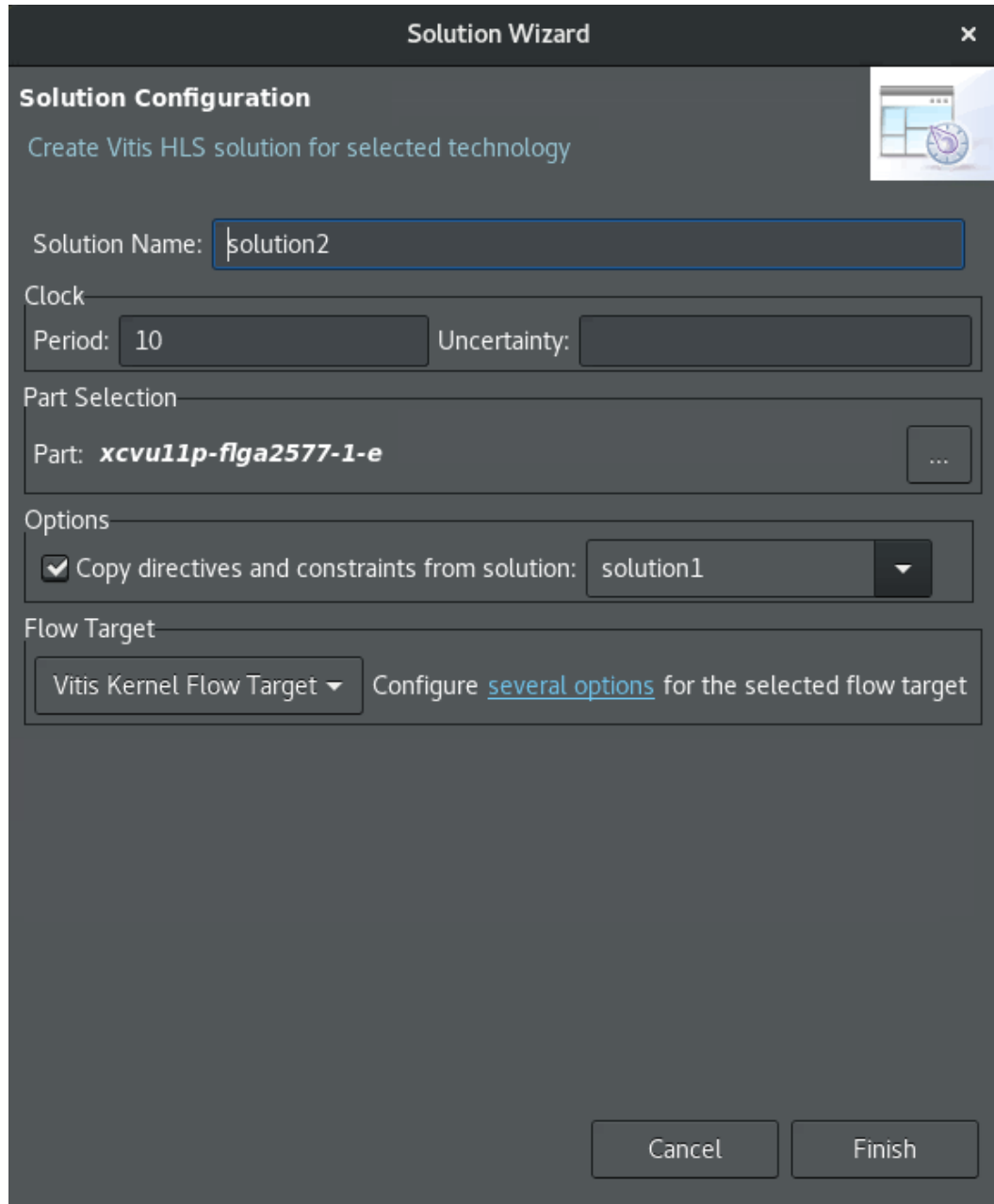
Figure 44: Solution Wizard
