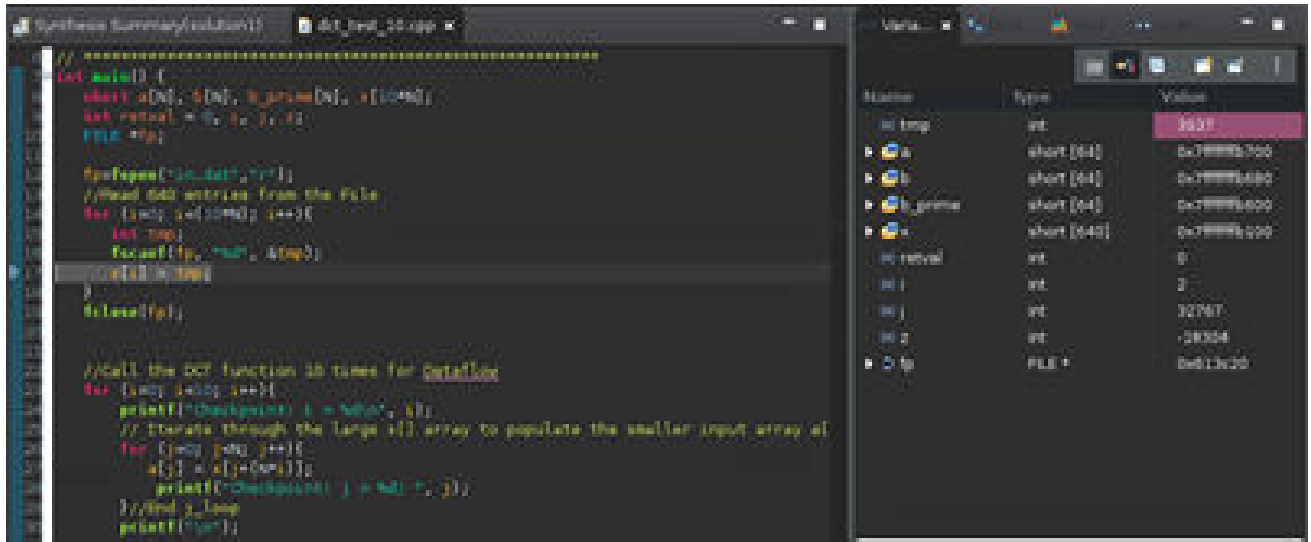
Figure 26: Monitoring Variables
