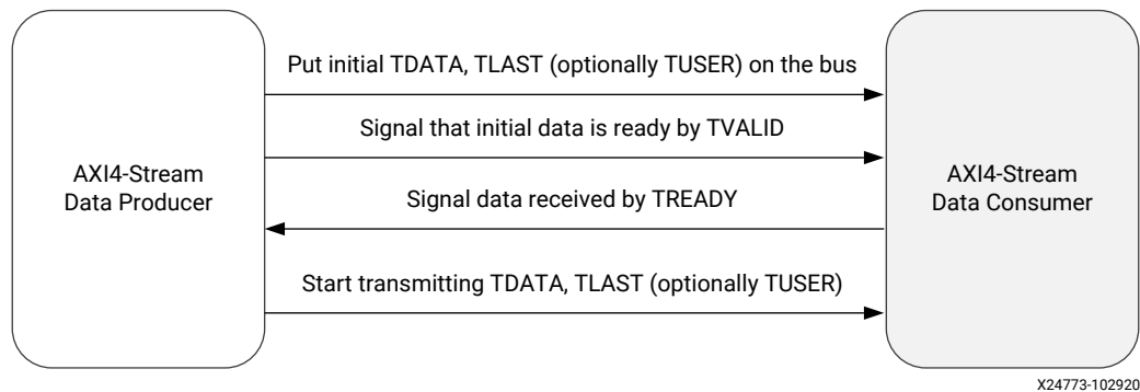
Figure 64: AXI4-Stream Handshake
