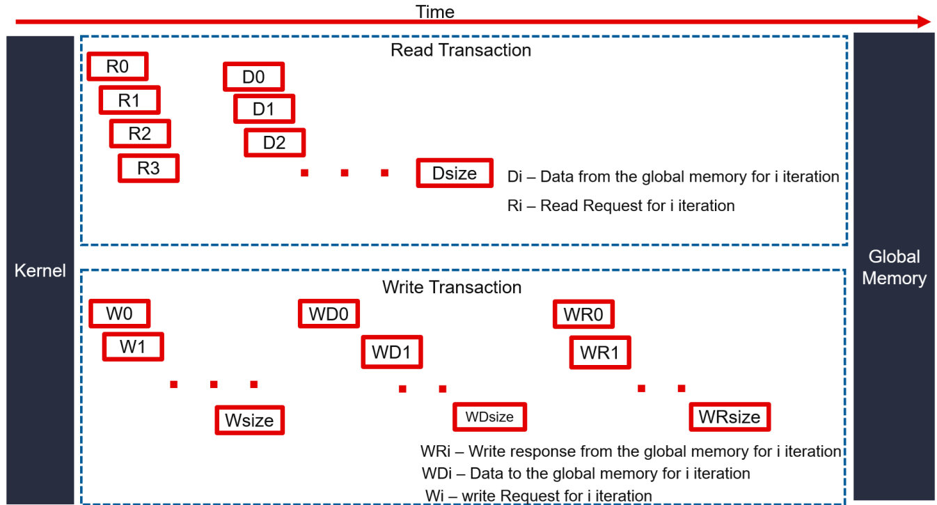
Figure 103: Pipeline Burst
