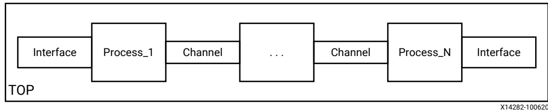
Figure 95: Parallel Process Architecture
