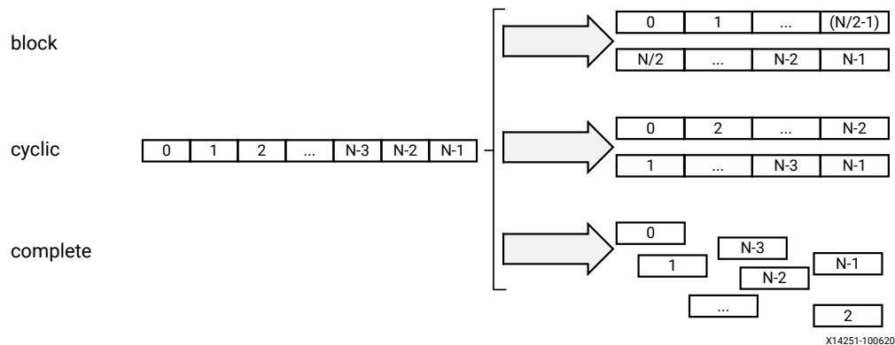
Figure 90: Array Partitioning
