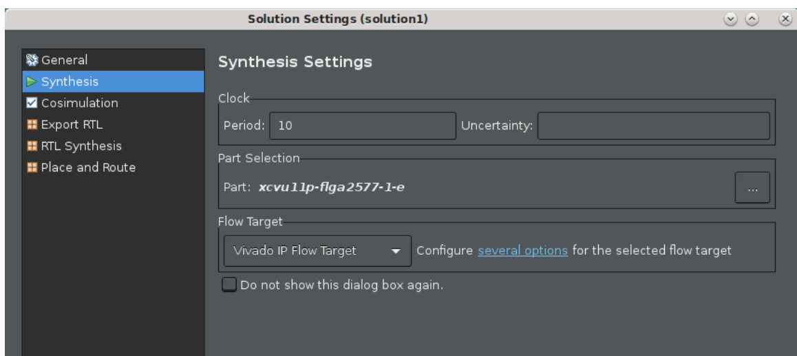
Figure 21: Synthesis Settings Page
