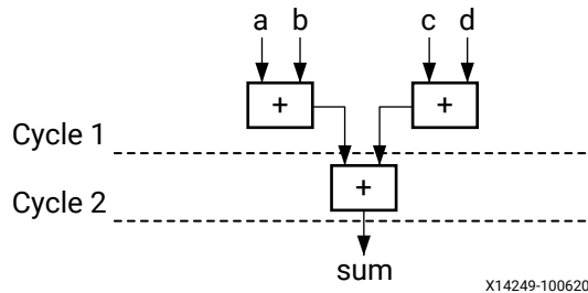
Figure 101: Adder Tree After Balancing
