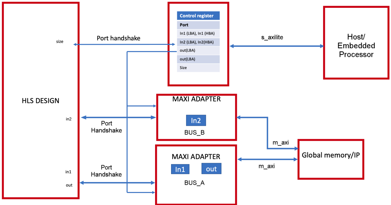
Figure 70: 2 MAXI Bundles
