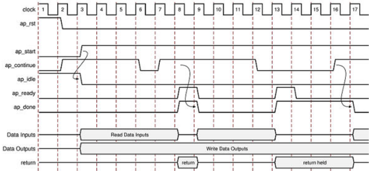
Figure 82: Behavior of ap_ctrl_chain Interface
