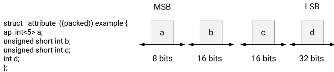
Figure 55: Packed Struct Implementation
