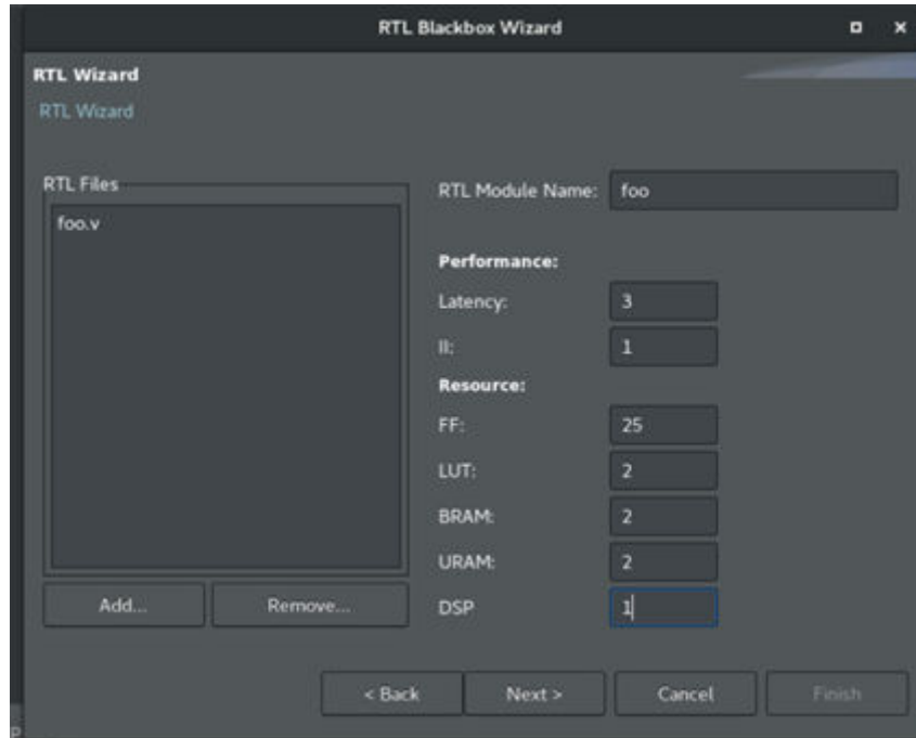
Figure 124: RTL Blackbox Wizard
