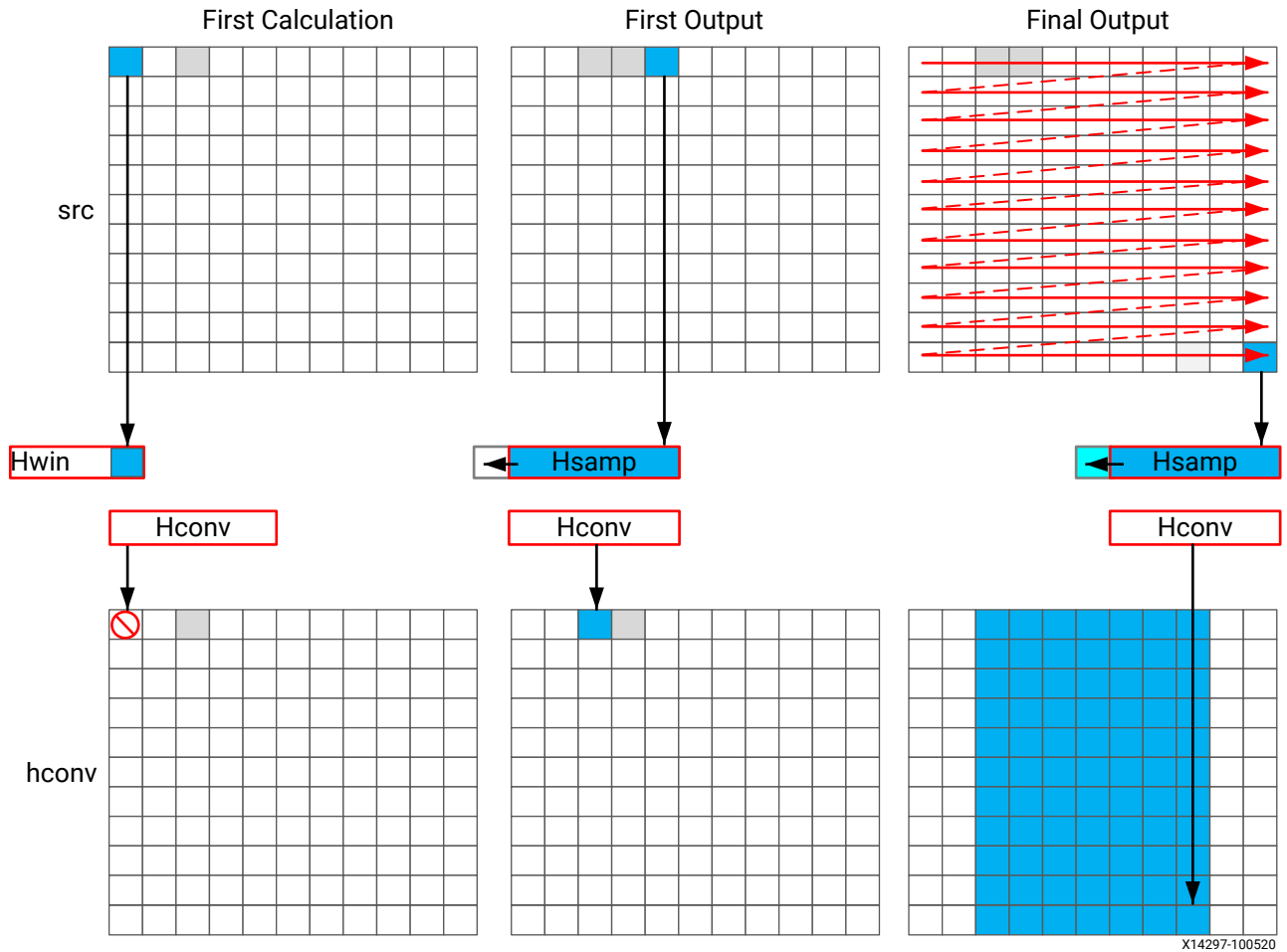
Figure 60: Streaming Horizontal Convolution
