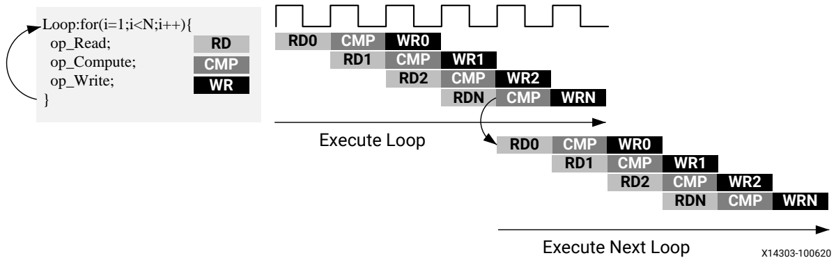
Figure 87: Loop Pipelining with Rewind Option
