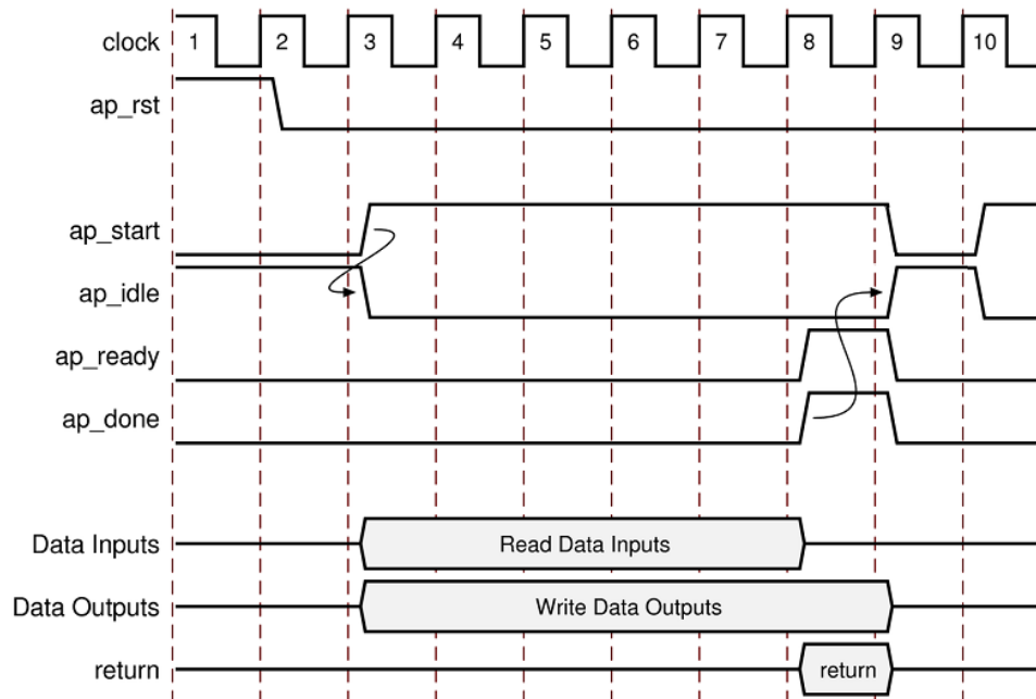
Figure 77: RTL Port Timing with Default Synthesis
