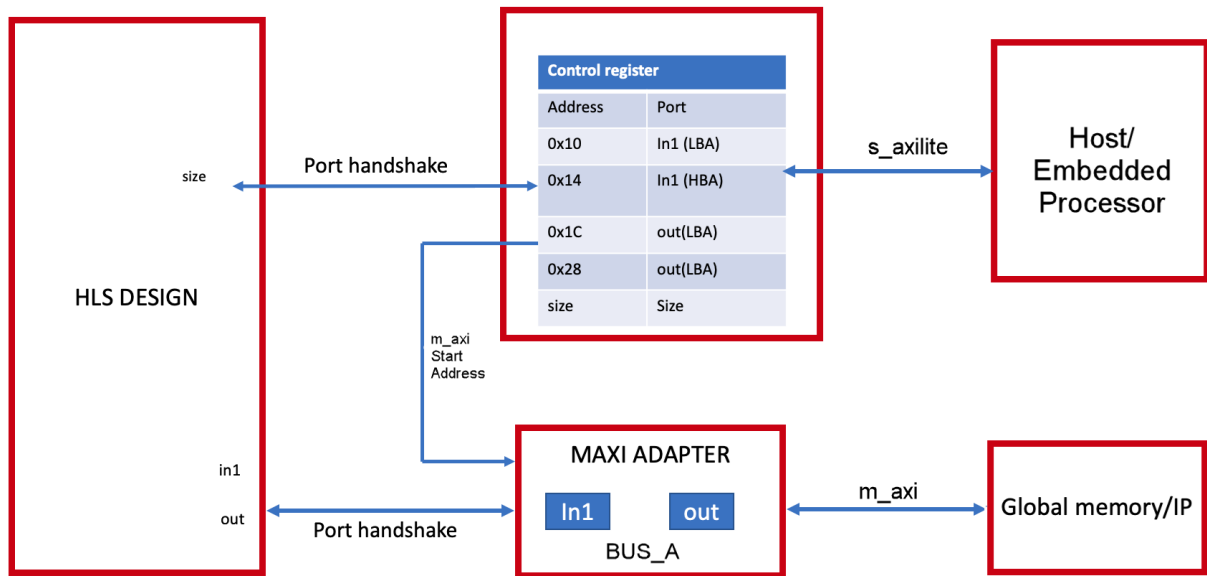
Figure 69: MAXI and S_AXILITE
