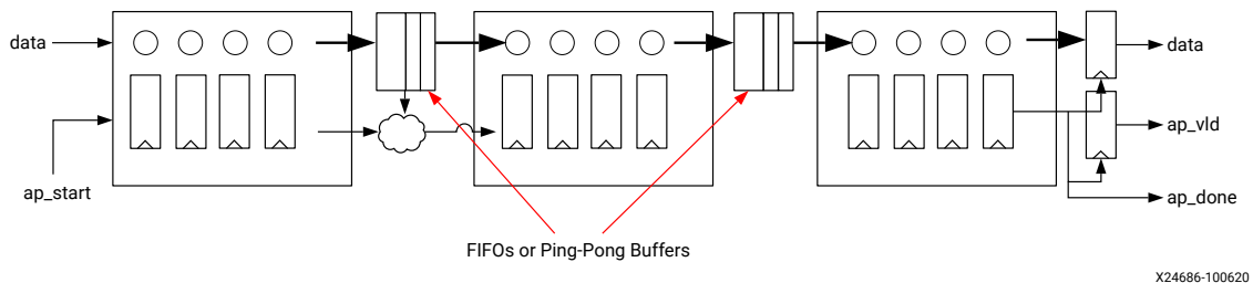
Figure 97: Structure Created During Dataflow Optimization
