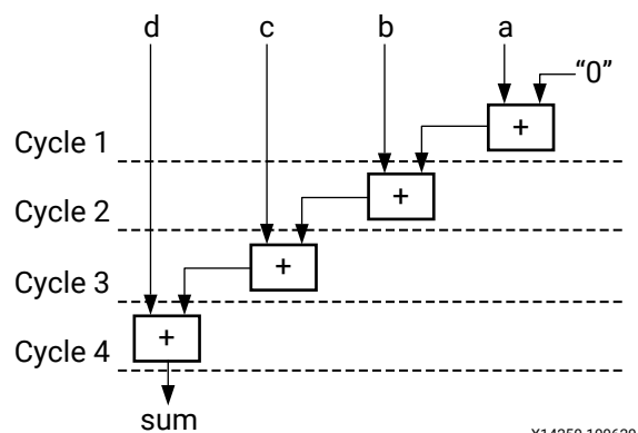
Figure 100: Adder Tree
