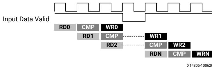
Figure 88: Loop Pipelining with Stall
