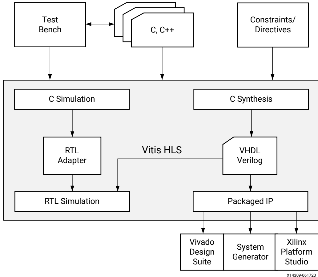
Figure 18: Vitis HLS Design Flow
