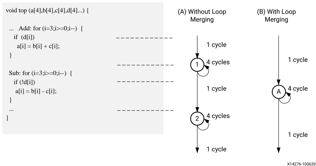
Figure 98: Loop Directives
