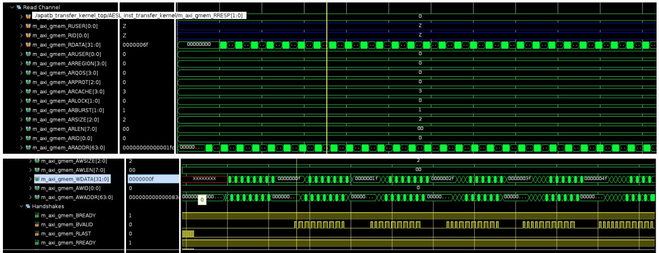
Figure 112: Performance Impacts
