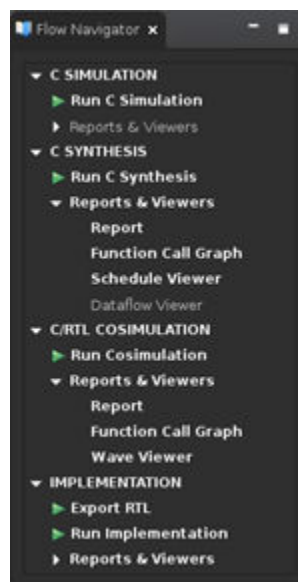
Figure 23: Flow Navigator
