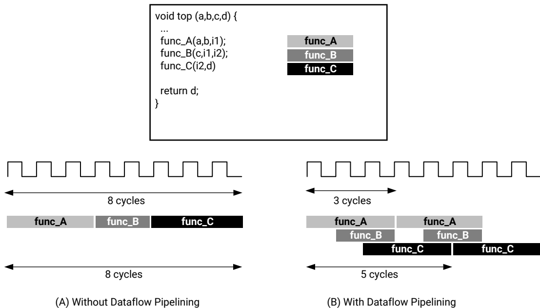
Figure 127: DATAFLOW Pragma
