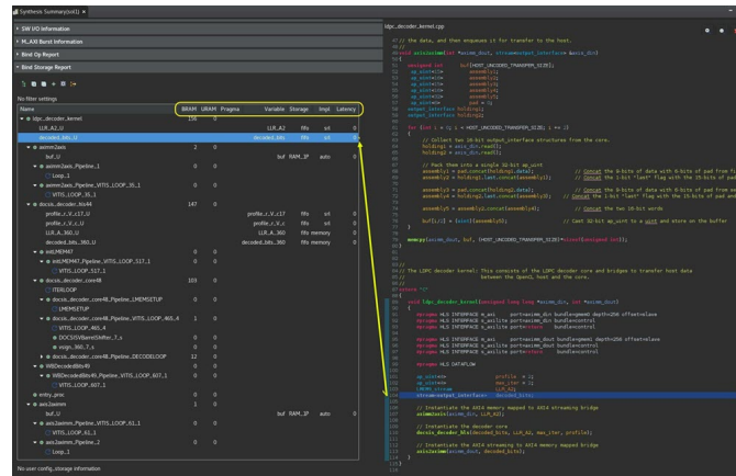
Figure 35: Synthesis Summary
