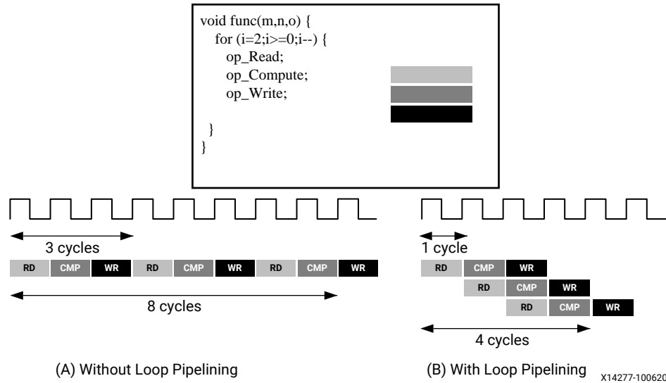
Figure 85: Loop Pipelining
