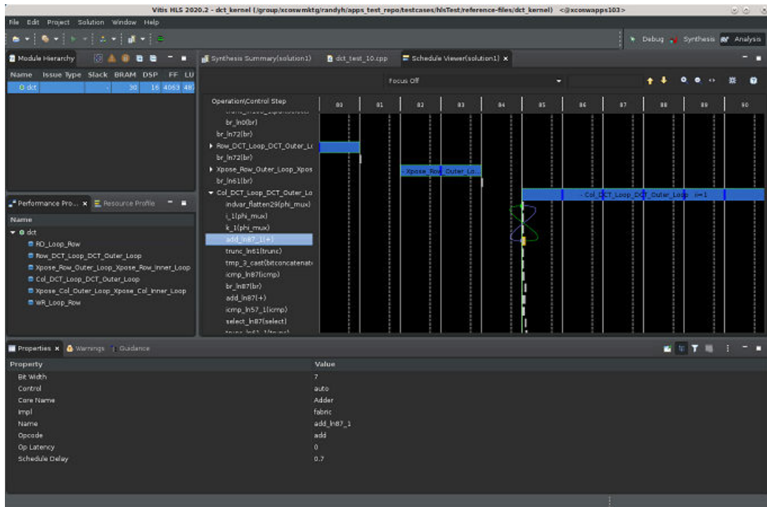
Figure 37: Schedule Viewer
