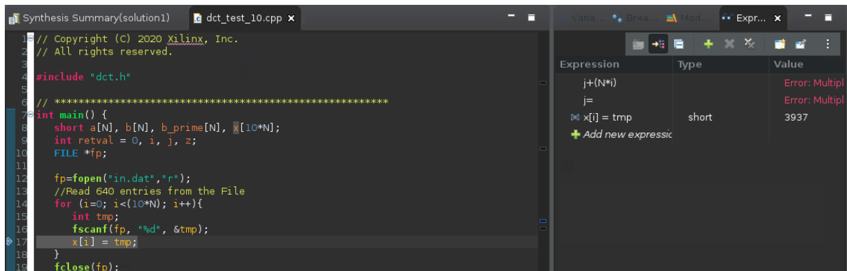
Figure 27: Monitoring Expressions
