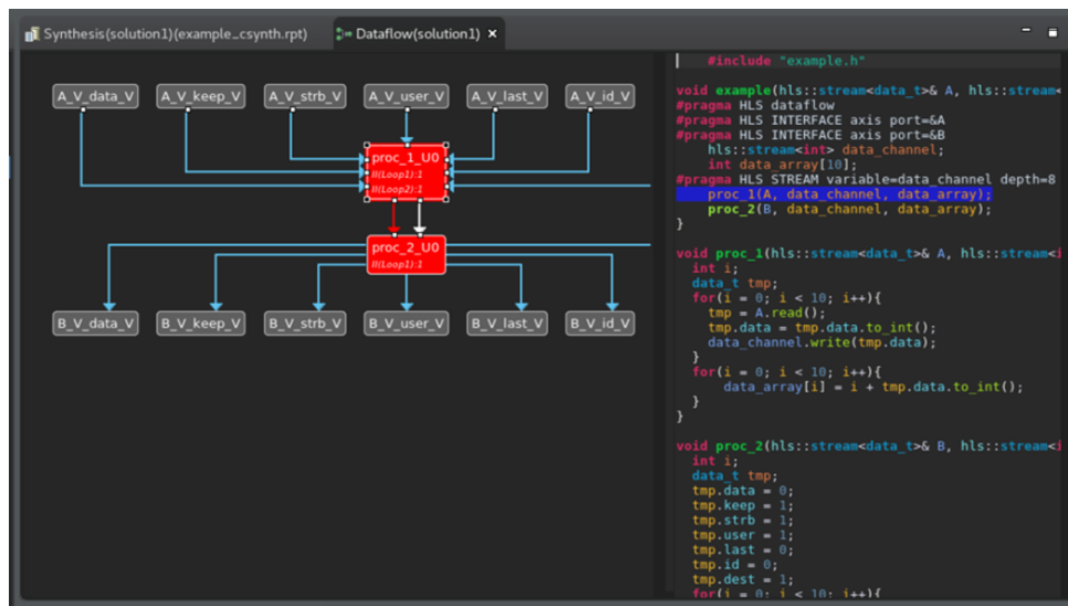
Figure 49: Deadlock Viewer
