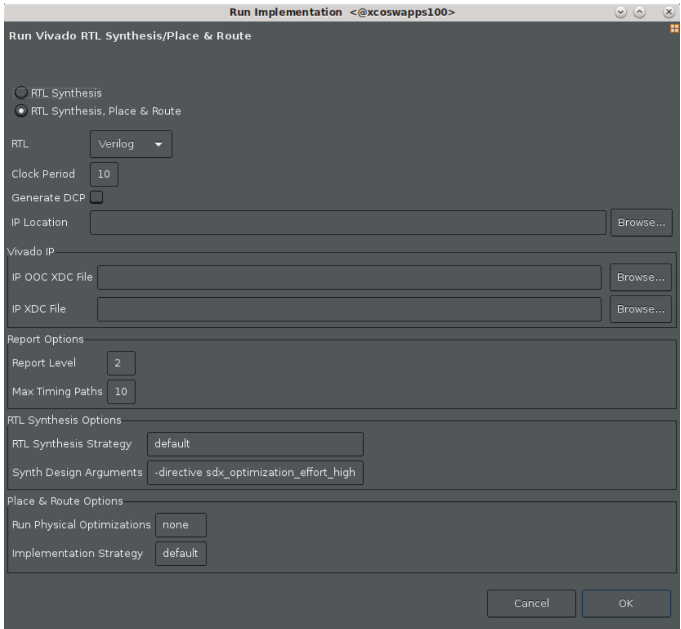
Figure 51: Run Implementation
