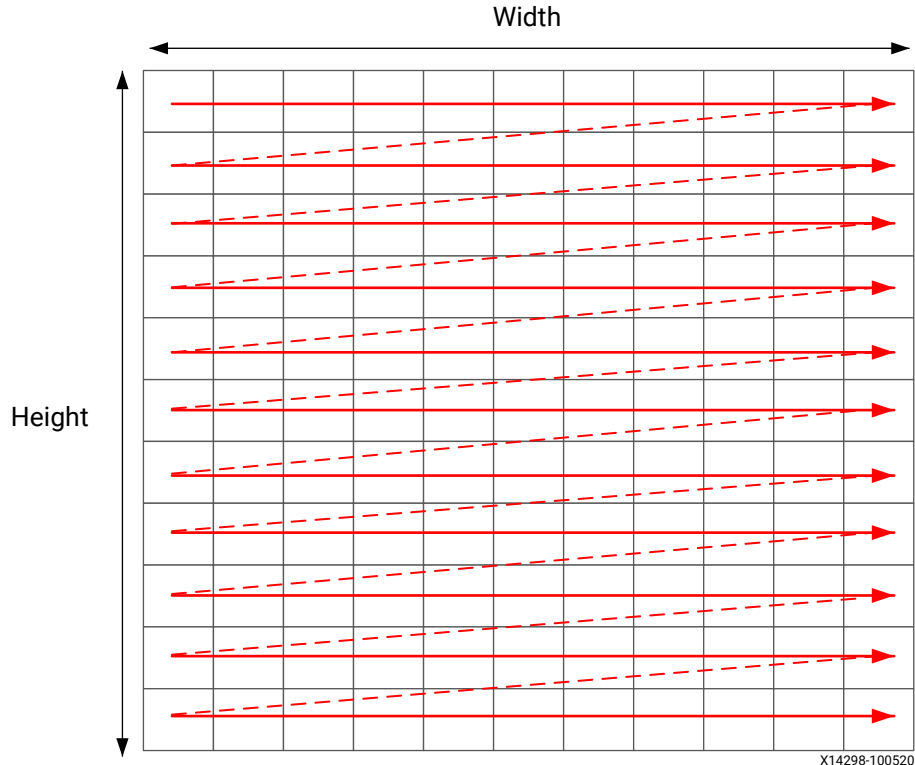
Figure 59: Raster Scan Order
