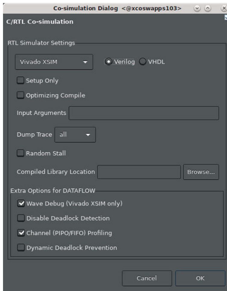
Figure 45: Co-Simulation Dialog Box
