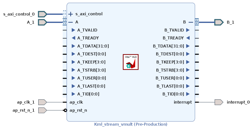
Figure 76: AXI4-Stream Interfaces with Side-Channels
